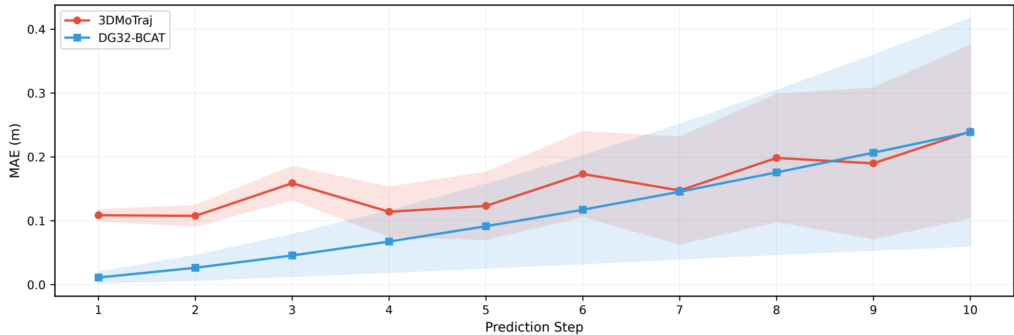
Per-Step Error Progression (Mean \pm Std)
